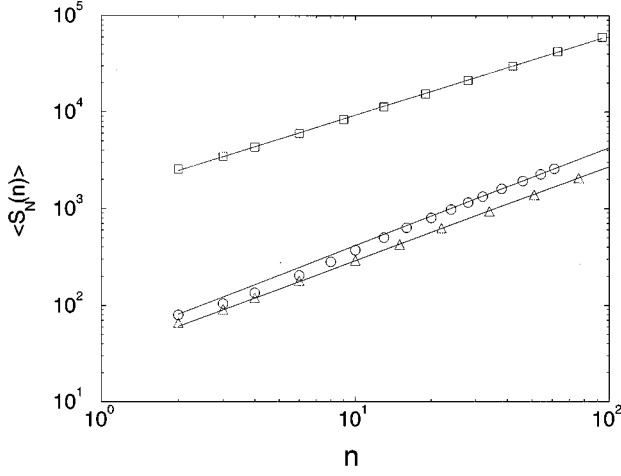
FIG. 4. The n dependence of the function \langle S_N(n) \rangle near the crossover between the regimes N^{2/(2+\alpha)}n^{2/\alpha} and n \ln(N/\ln n) , see Table I for the case \alpha > 2 . In the case \alpha = 2.5 ( \square ) we see the behavior before the crossover, \langle S_N(n) \rangle \propto n^{2/\alpha} : the fitted line slope is 0.82 \approx 2/\alpha = 0.8 . The plot for the case \alpha = 7.0 ( \circ ) shows partially (small n ) the crossover regime and the slope for the large n is about 1.0. In the plot for \alpha = 8.0 ( \triangle ) the crossover regime does not appear and \langle S_N(n) \rangle \propto n : the fitted slope is about 0.97.
