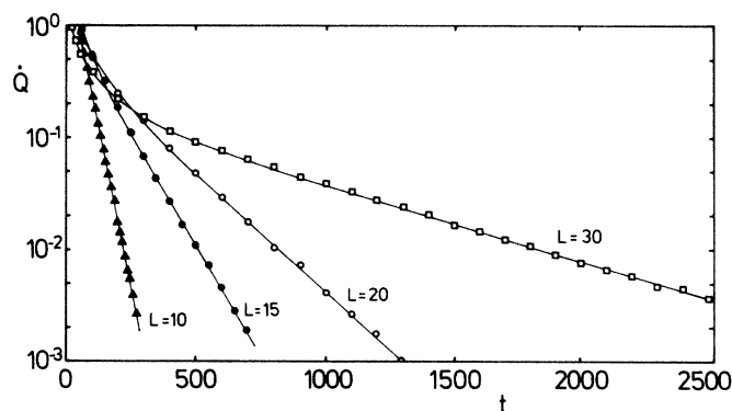
FIG. 2. Test of Eq. (4a), P(L, t) \sim e^{-t/\tau} ; shown in a semilogarithmic plot of \dot{Q} \equiv -\dot{P} as a function of time for c_F=0.1 , c_T(0)=0.2 , with L=10 ( \Delta ), 15 ( \bullet ), 20 ( \circ ), and 30 ( \square ). The results are based on 2000 runs (or more) for each L value.
