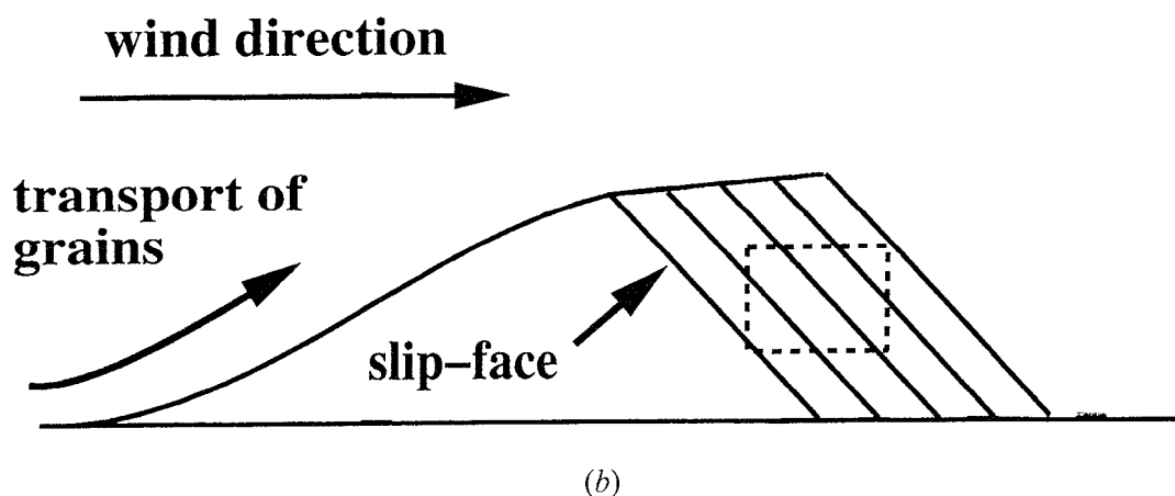
Figure 4. (b) Schematic representation of the formation of a slip face of a dune. After an incipient dune is formed, the wind moves sand from the upstream side to the top, and dune avalanches ( grain flow ) begin. This kind of large-scale sedimentary structure occurs on length scales ranging from tens of centimetres to tens of metres and is characterized by avalanching of grains (Bagnold 1941) (as opposed to small-scale ripple formations which are typically 1 cm in amplitude (Forrest and Haff 1992) and are mainly dominated by grainfall ). Grain flow (avalanches) and grain fall (small ripples) lead to size segregation of opposite sign; in grain flow, the large grains tend to be on the bottom of the dune while, in grainfall, the large grains tend to be on the top (see, for example, figure 3 of Anderson and Bunas (1993)). Grain flow also occurs in other sedimentary systems, such as fluvial, but in that case the geological process is modified by the turbulent water flow.
