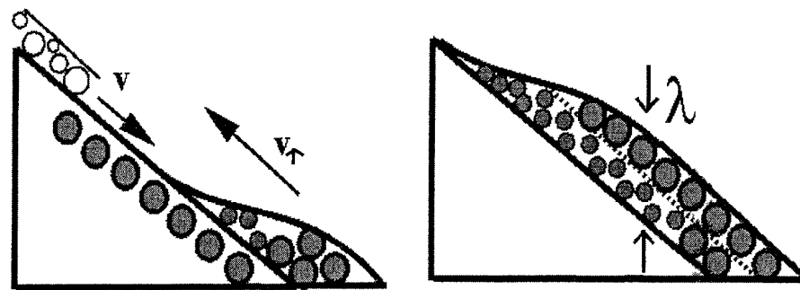
Figure 2. Description of the formation of the layers and ‘kink’ mechanism.
